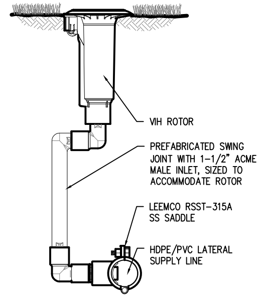
1 RSST-315A Swing Joint
