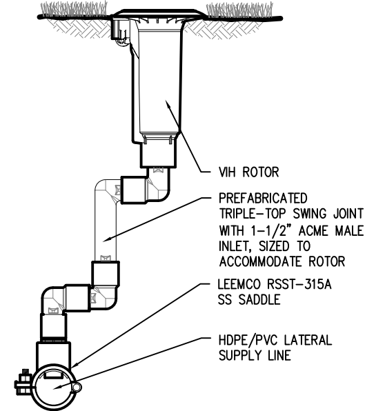
1 RSST-315A Triple-Top Swing Joint
