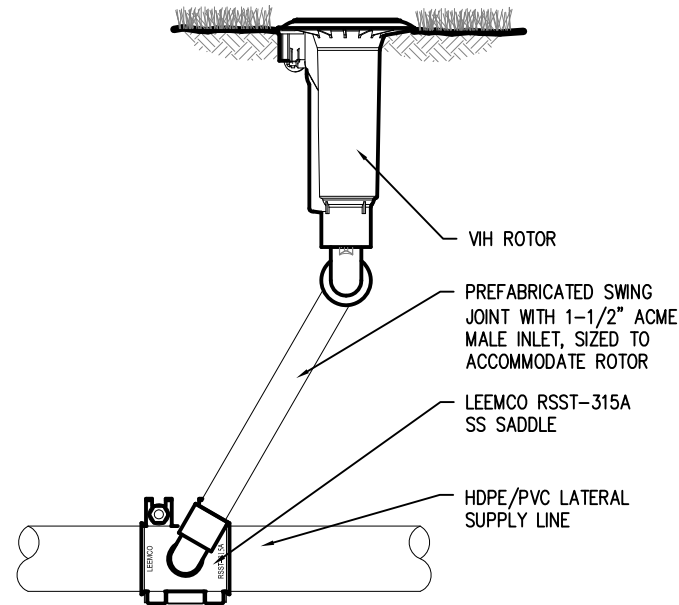
1 RSST-315A Swing Joint
