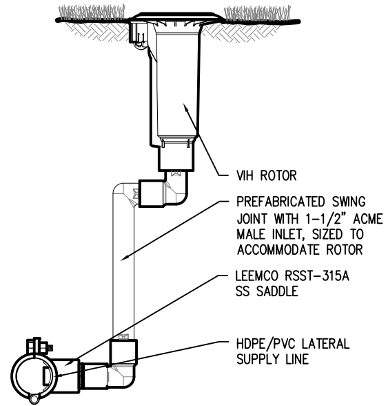
1 RSST-315A Swing Joint
